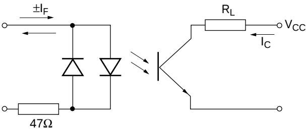
Figure 2. Test circuit—SFH628A
