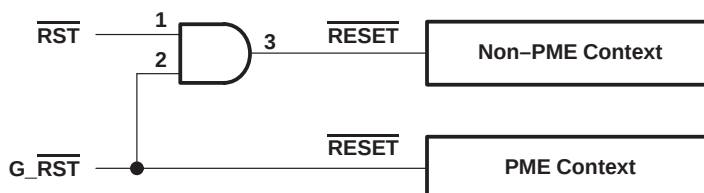
Figure 6. TSB12LV23 Reset Block Diagram
