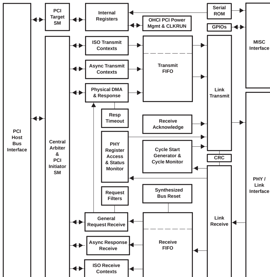
Figure 1. TSB12LV23 Block Diagram
