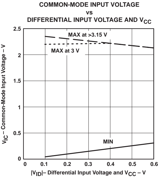
Figure 3. Maximum V_{IC} versus V_{ID} and V_{CC}
