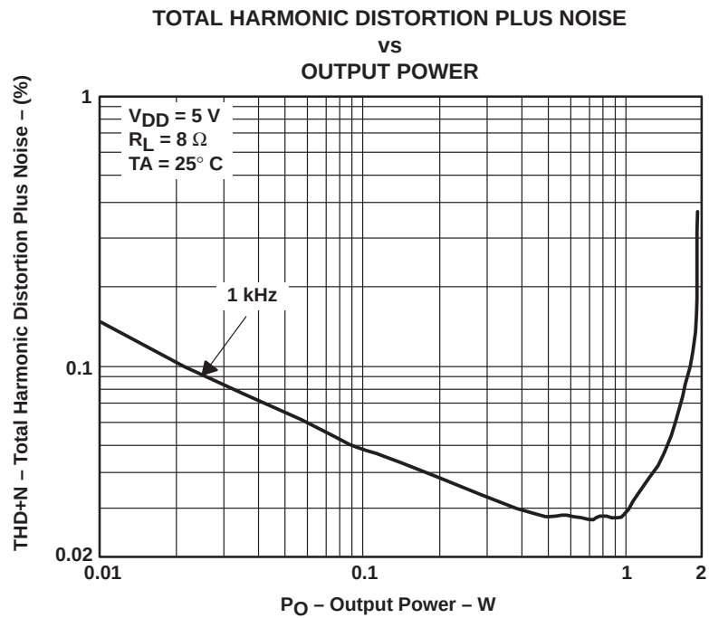
Figure 3–13. Class-D Amplifier Distortion versus Output Power at 8 \Omega
