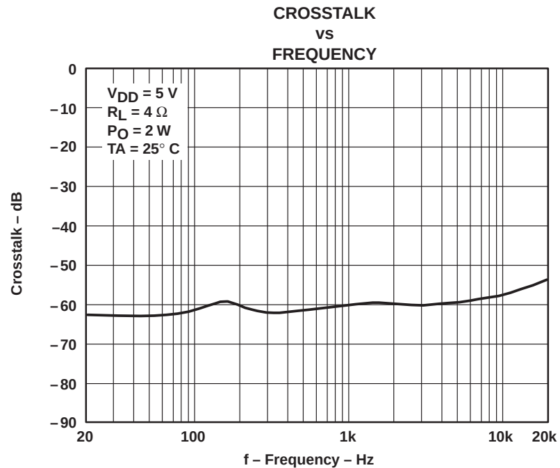
Figure 3–16. Class-D Amplifier Crosstalk versus Frequency at 2 W Into 4 \Omega
