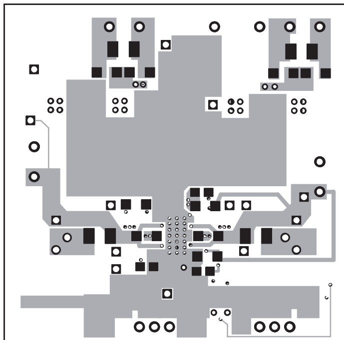
Figure 3–24. TPA005D12 Class-D EVM Bottom Layer
