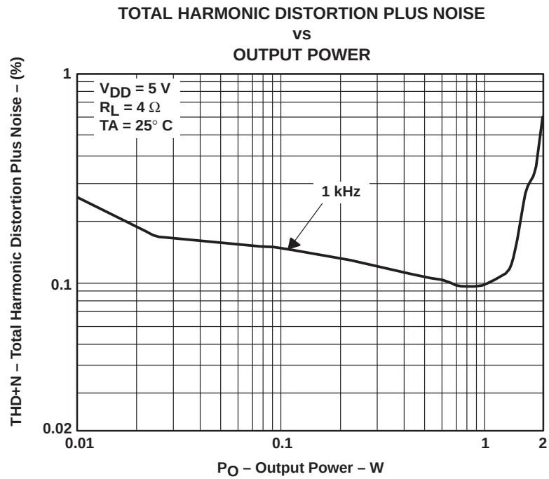
Figure 3–12. Class-D Amplifier Distortion versus Output Power at 4 \Omega
