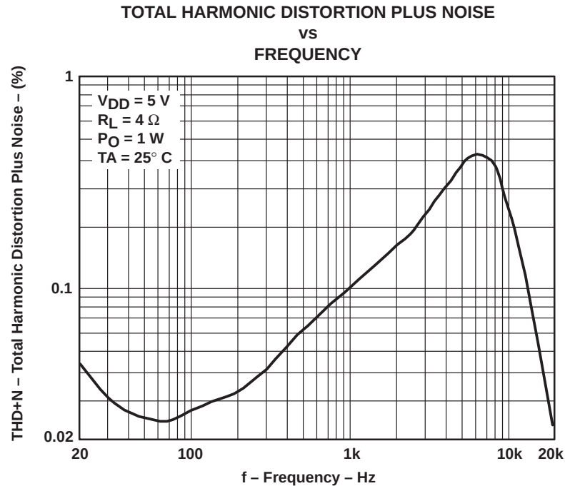
Figure 3–14. Class-D Amplifier Distortion versus Frequency at 1 W Into 4 \Omega
