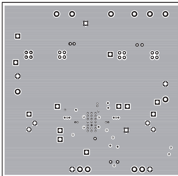
Figure 3–23. TPA005D12 Class-D EVM Third Layer
