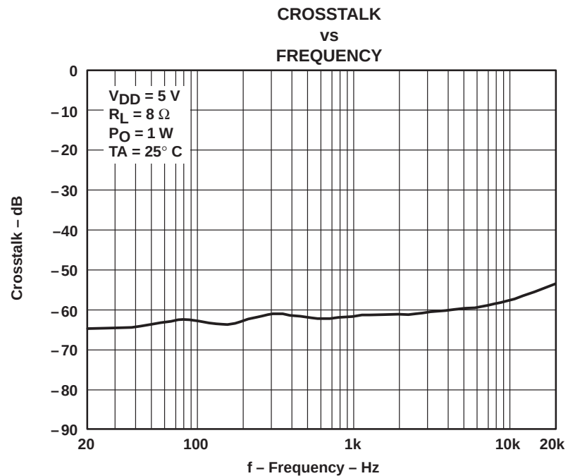
Figure 3–17. Class-D Amplifier Crosstalk versus Frequency at 2 W Into 8 \Omega
