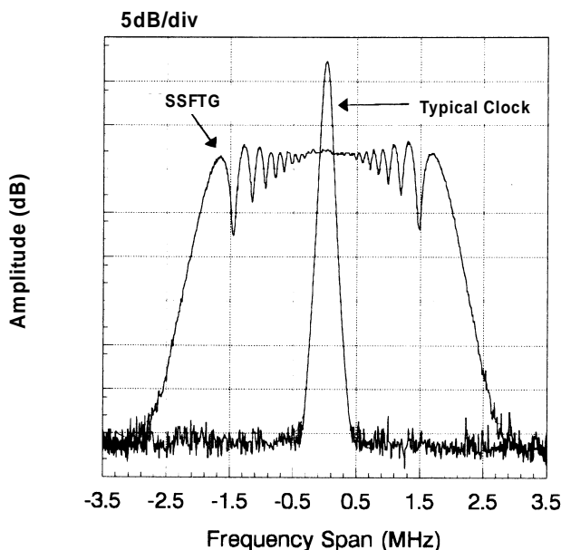
Figure 3. Clock Harmonic with and without SSCG Modulation Frequency Domain Representation
