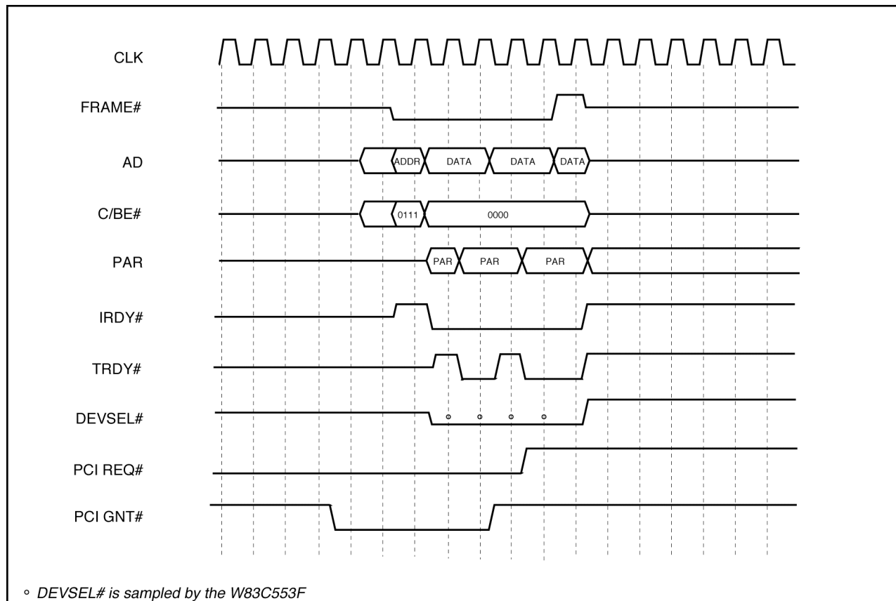
Figure 3-12. Preemption Timing
