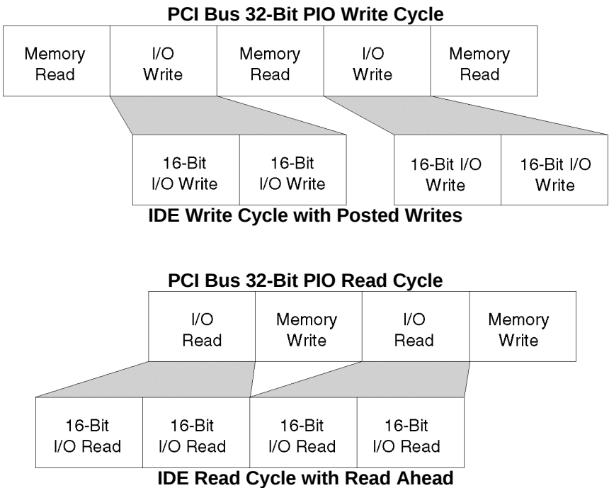
The two drawings shown above show the relationship between the PCI bus and the IDE interface.
