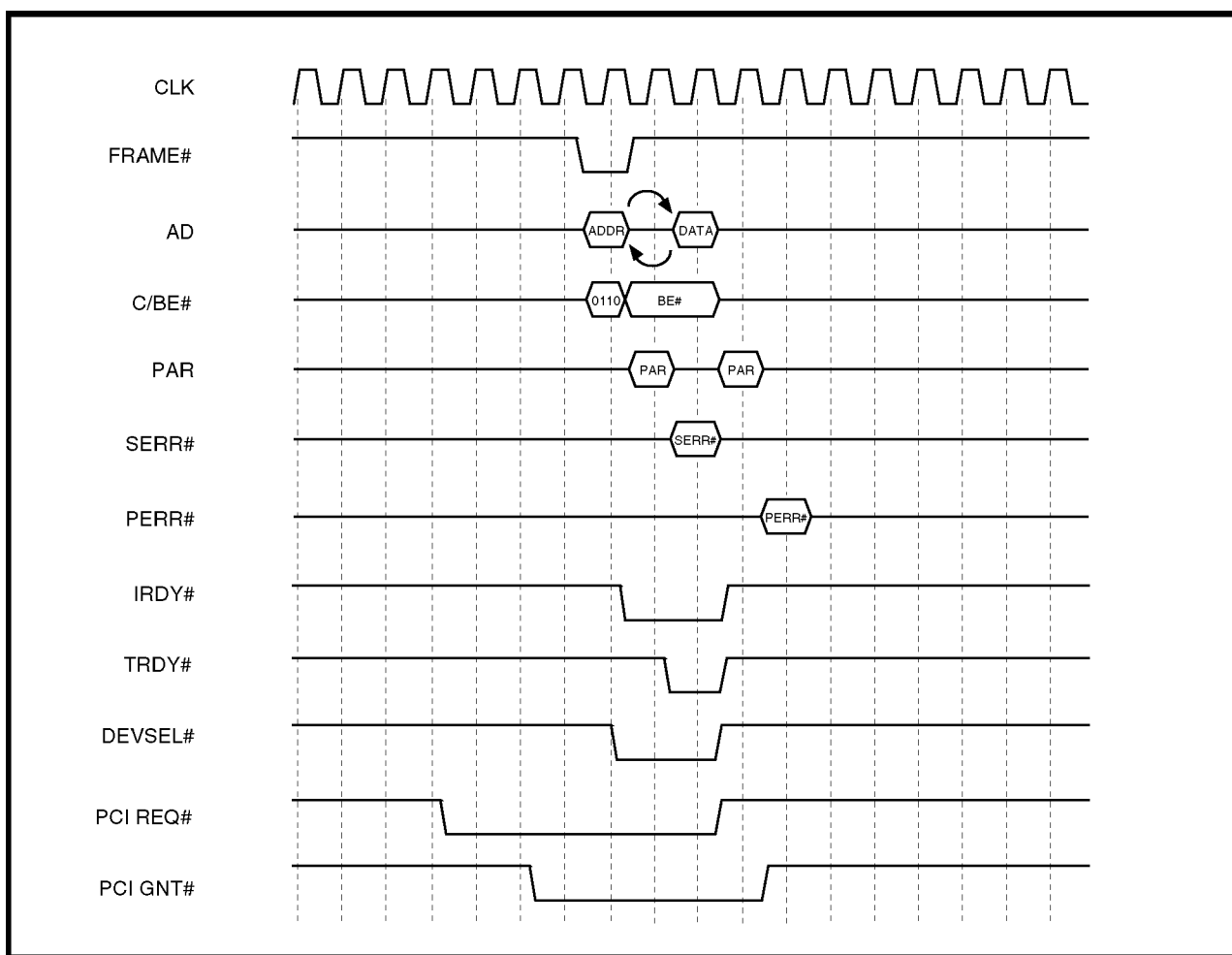
Figure 3-6. Master Memory Read Timing
