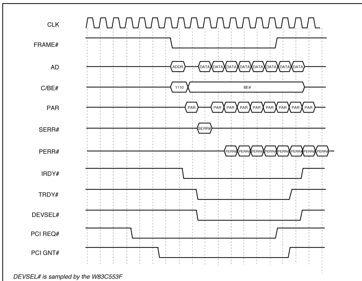
Figure 3-8. Master Memory Read Line Timing
