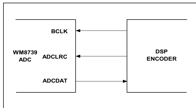
Figure 18 Slave Mode
