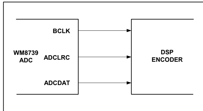
Figure 17 Master Mode
