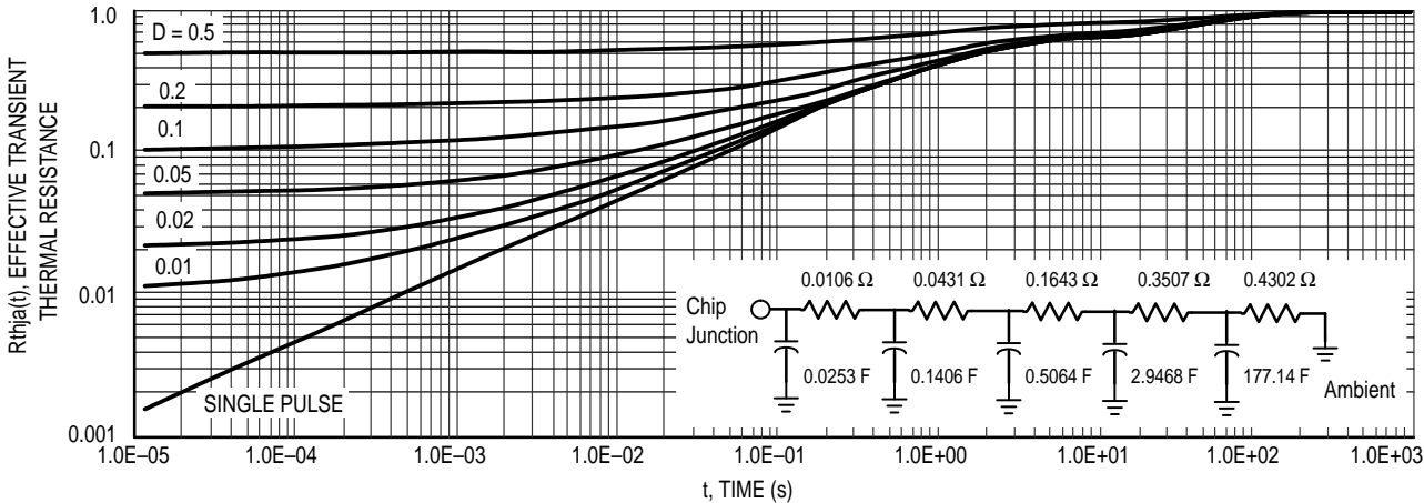
Figure 14. Thermal Response
