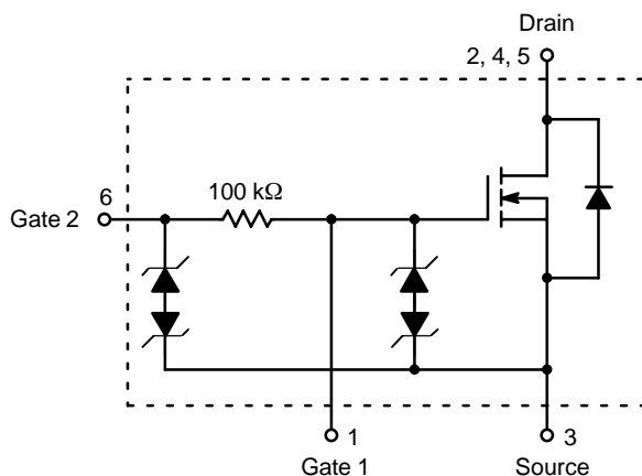
Figure 1. Block Diagram
