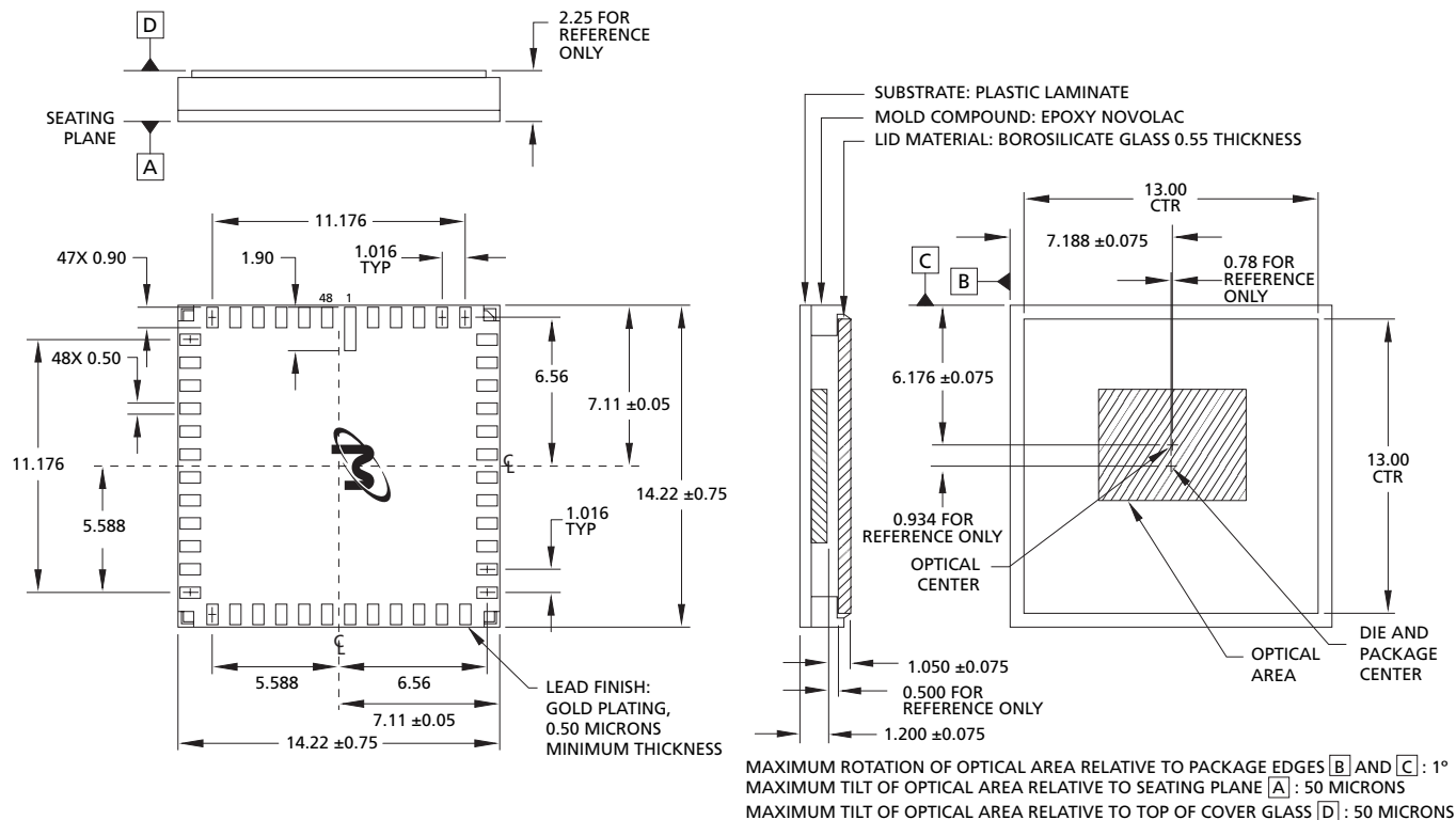
Figure 30: 48-Pin PLCC
