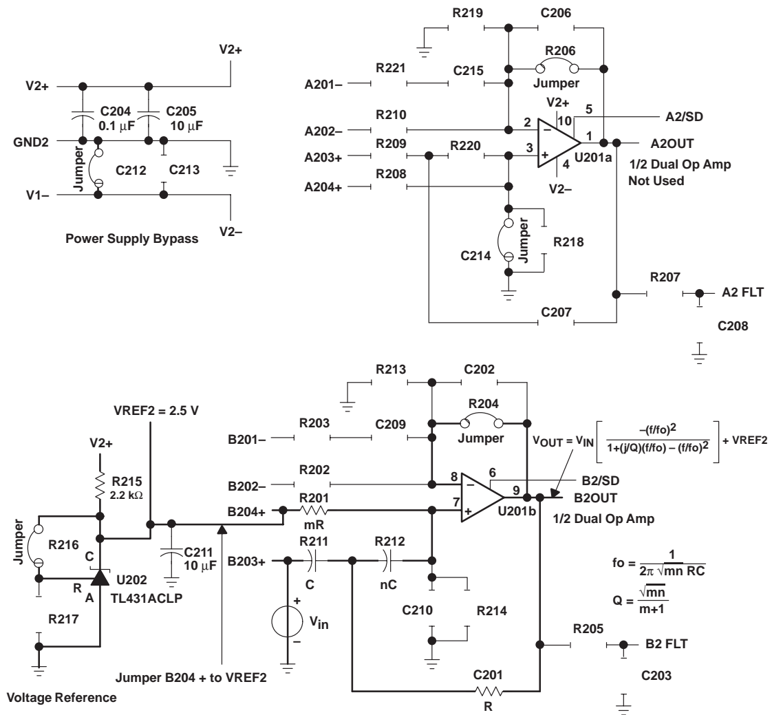
Figure 4–2. Sallen-Key High-Pass Filter with Single Supply Using Area 200
