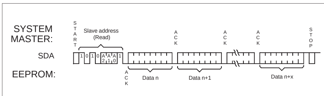
Figure D-9. EEPROM Sequential Read Operation
