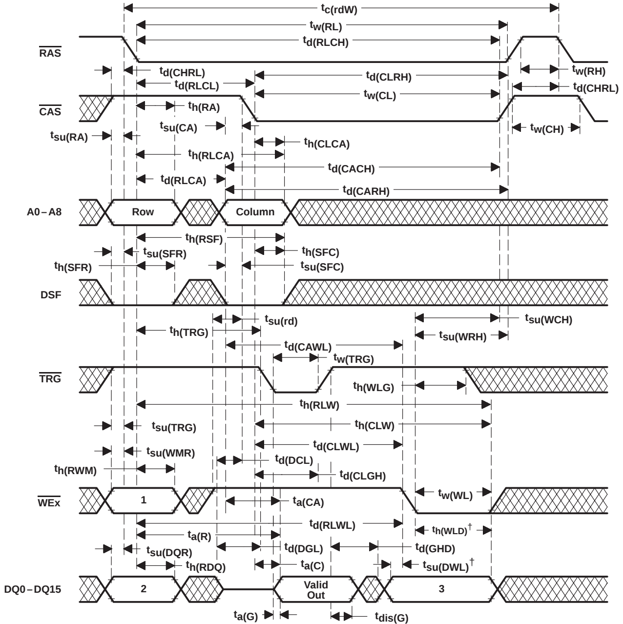
Figure 34. Read-Modify-Write-Cycle Timing
