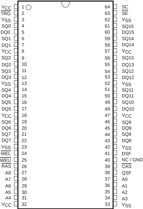
DGH PACKAGE (TOP VIEW)
