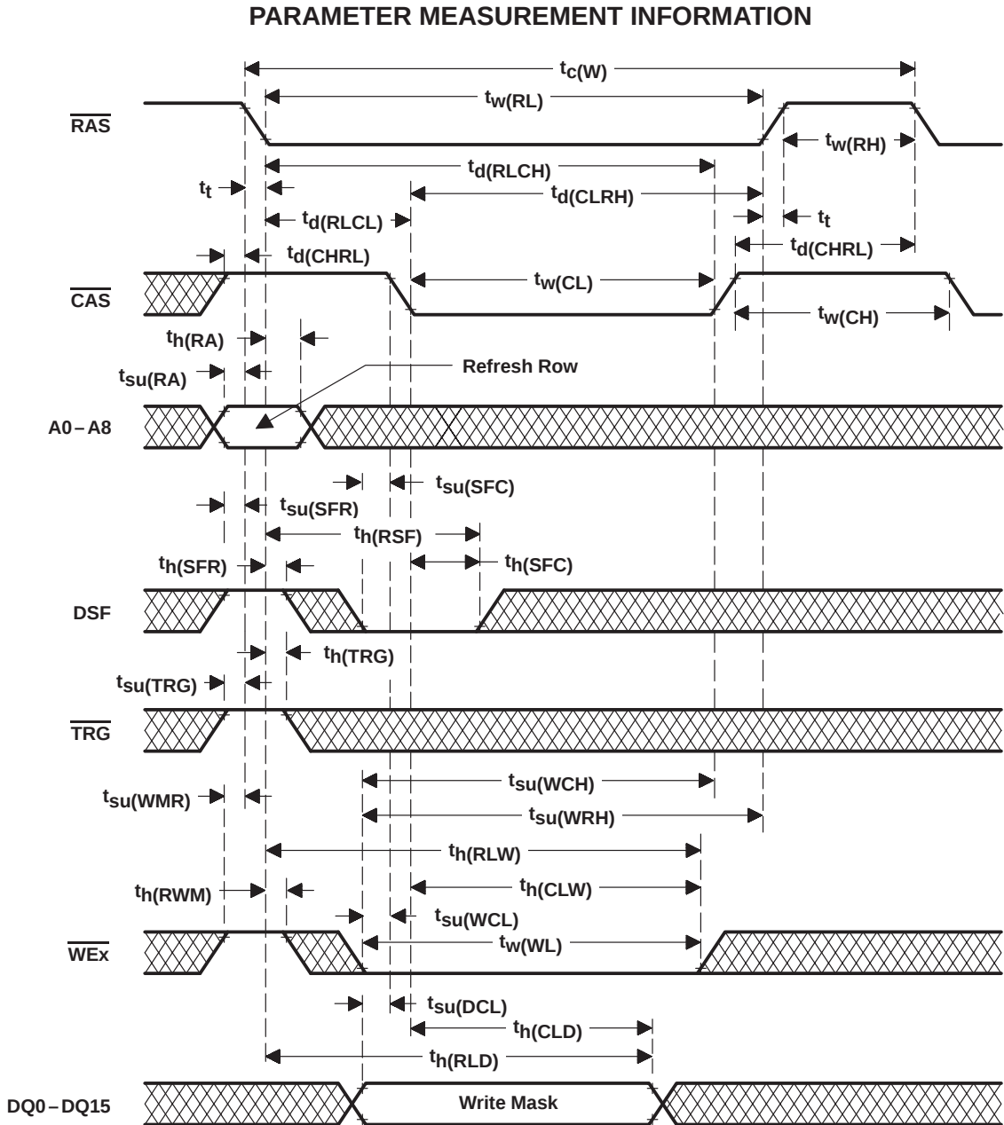
Figure 37. Load-Write-Mask-Register-Cycle Timing (Early-Write Load)
