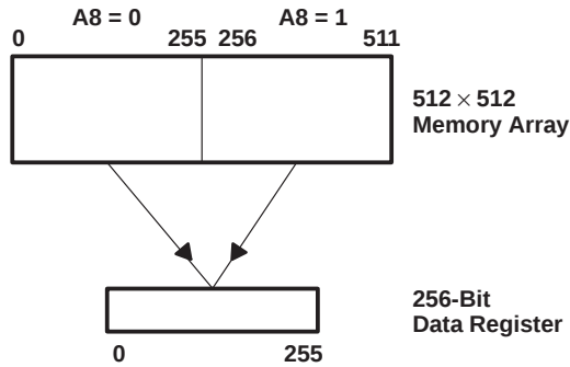
Figure 18. Full-Register-Transfer Read
