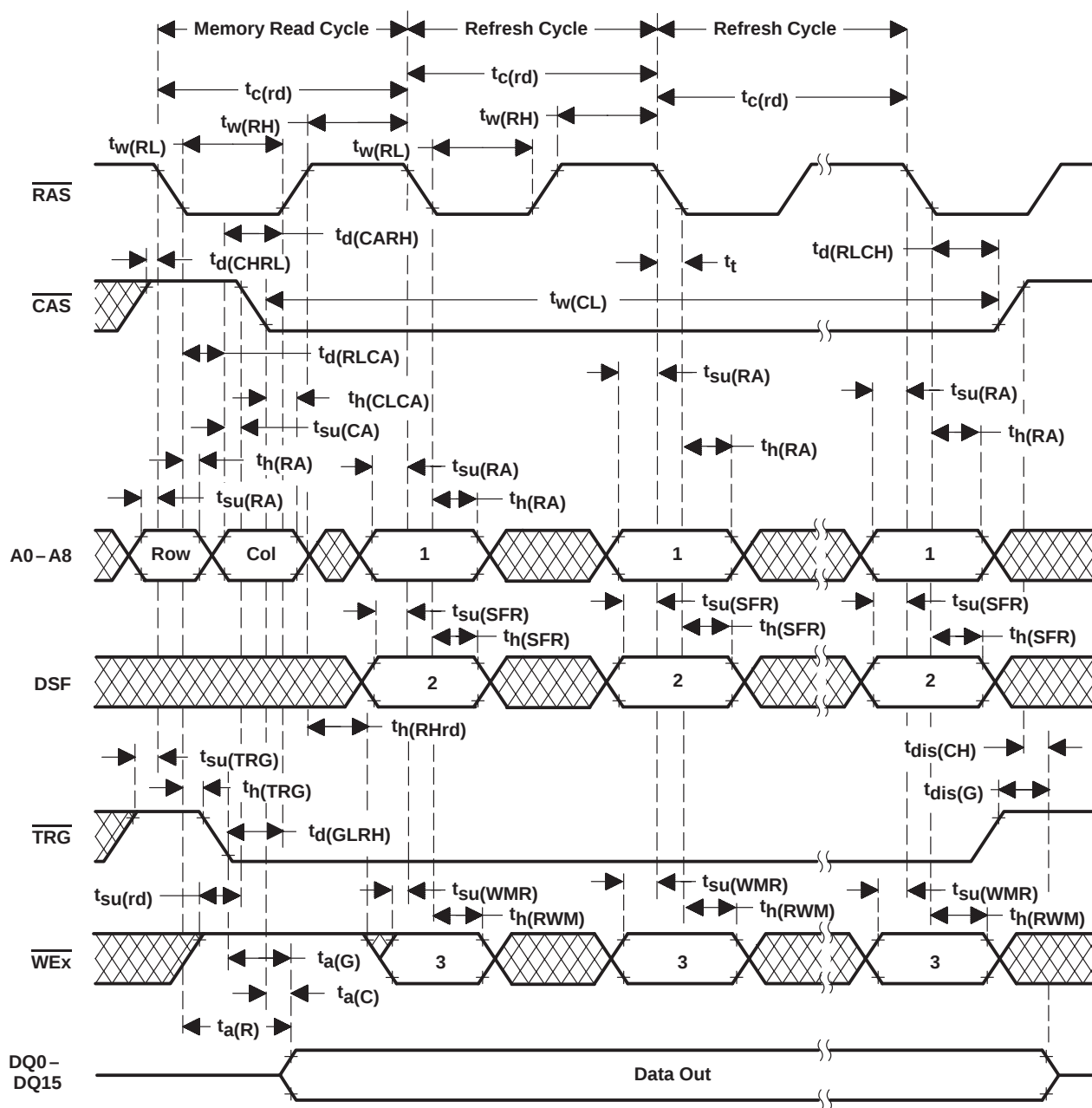
Figure 49. Hidden-Refresh-Cycle Timing
