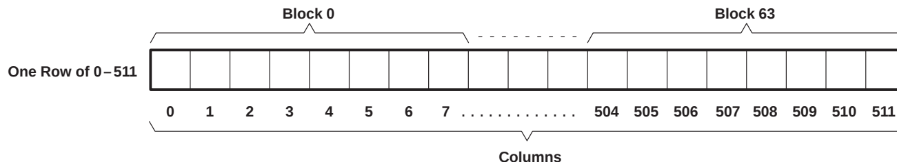
Figure 15. 8-Column-Block Column-Organization
