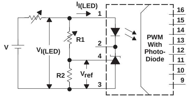
Figure 3. \Delta V_{ref}/\Delta V_{L(LED)} Test Circuit
