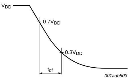
Fig 41. Definition of the fall time of the output signal
