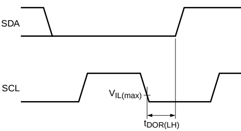
a. Data change from LOW to HIGH.
