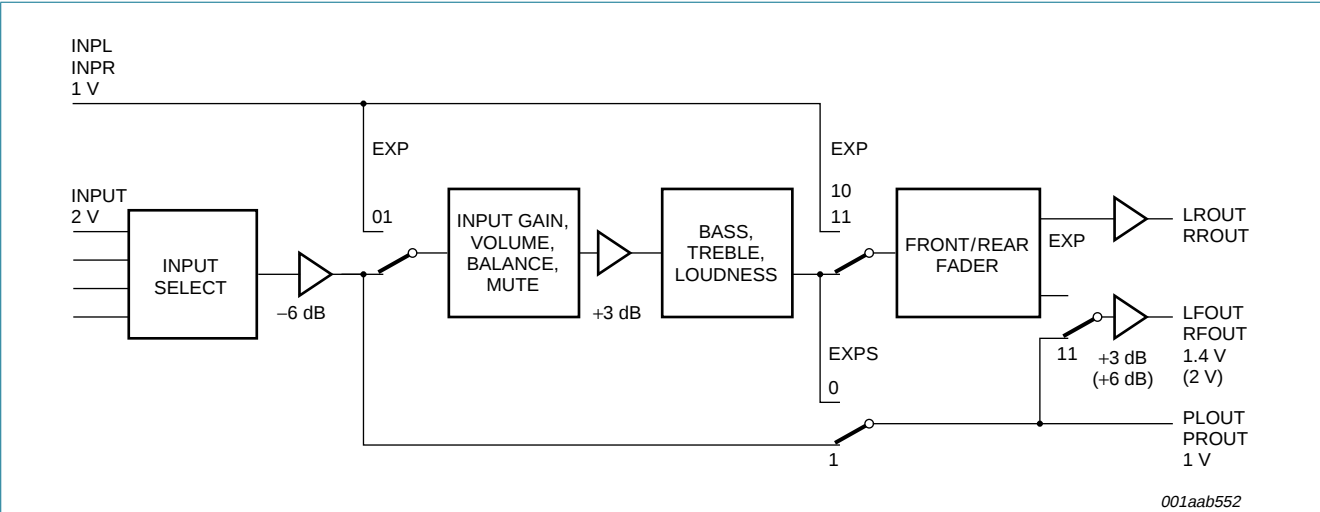
Fig 37. External processor connections
