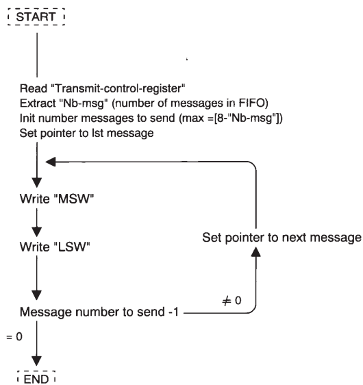
Figure 33 : Transmitter without interrupt flow-chart.
