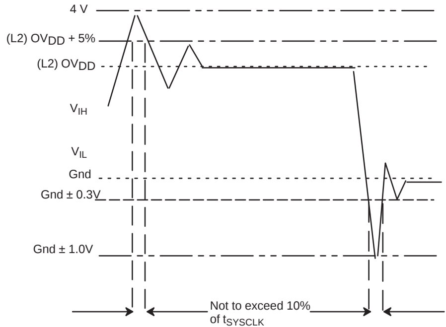
Figure 5. Overshoot/Undershoot Voltage
