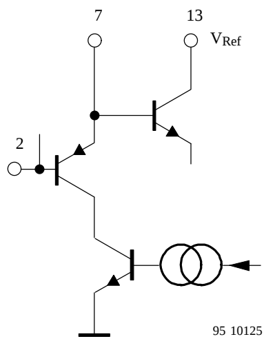
Figure 10. Pin 7 RC+
