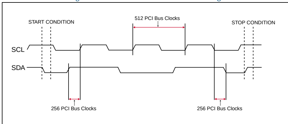
Figure 8: Serial EEPROM Waveforms and Timings
