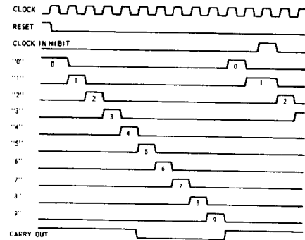
Fig. 2 - Timing diagram.
