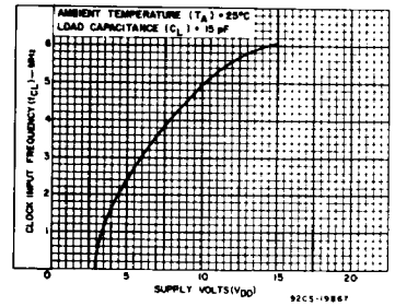
Fig. 7 — Typical clock input frequency vs. V_{DD} .
