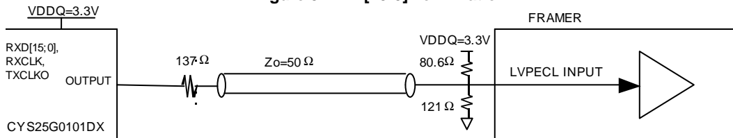
Figure 10. LVPECL-compliant Output Termination
