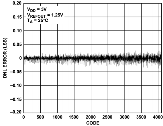
Figure 16. DNL—12-Bit DAC, 1.25 V Internal Reference
