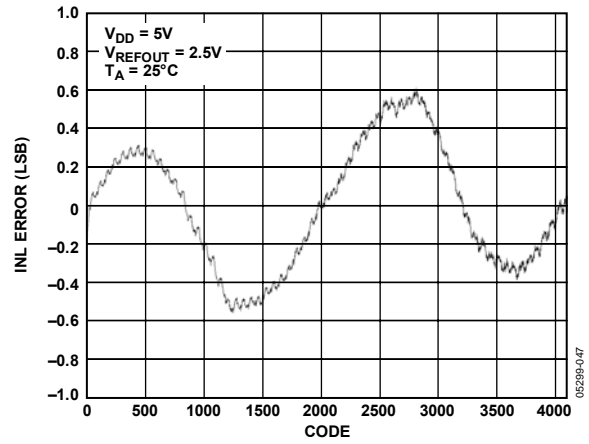
Figure 13. INL—12-Bit DAC, 2.5 V Internal Reference
