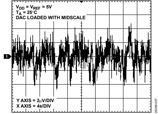
Figure 37. 0.1 Hz to 10 Hz Output Noise Plot, External Reference
