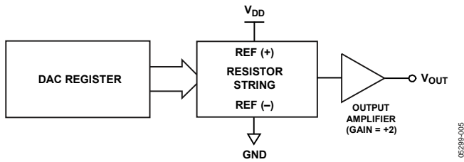
Figure 45. DAC Architecture
