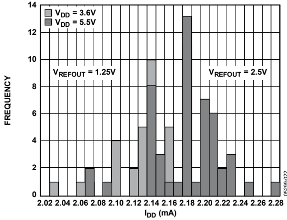
Figure 22. I_{DD} Histogram with Internal Reference
