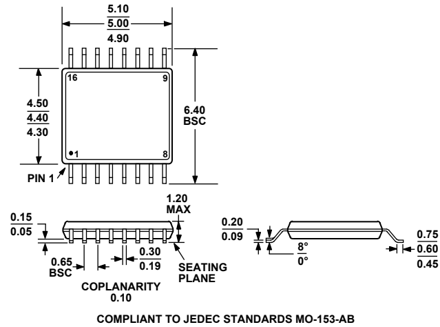
Figure 52. 16-Lead Thin Shrink Small Outline Package [TSSOP] (RU-16) Dimensions shown in millimeters
