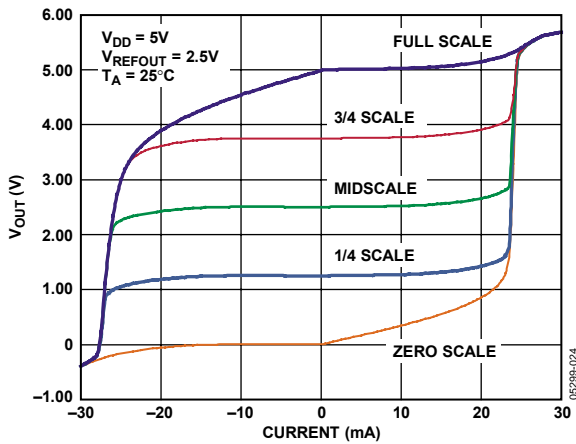
Figure 24. AD5678-2 Source and Sink Capability
