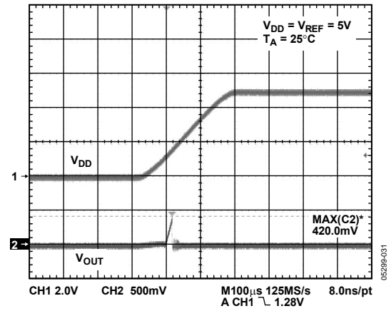
Figure 31. Power-On Reset to 0 V
