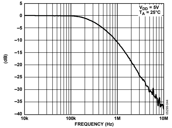
Figure 44. Multiplying Bandwidth
