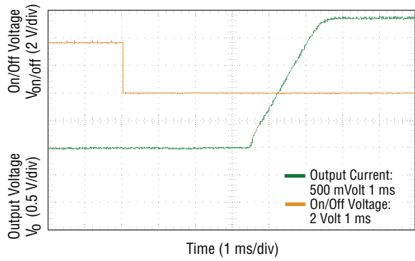
Fig. 17 Typical Start-up using Remote On/Off with Prebias ( V_{in} = 5 V_{dc} , V_o = 3.3 V_{dc} , I_o = 1 A , V_{bias} = 1 V_{dc} )
