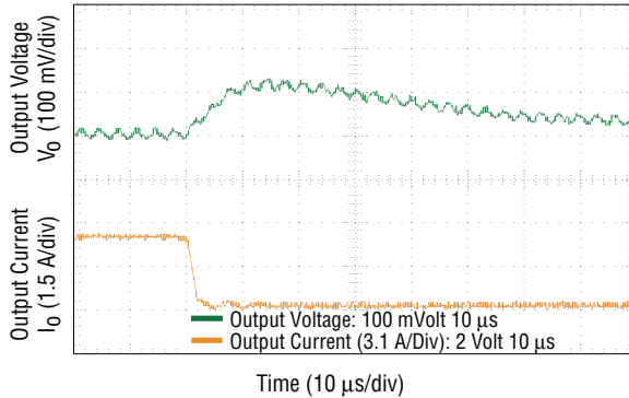
Fig. 13 Transient Response - 10 A - 5 A Step ( V_o = 3.3 V_{dc} , C_{ext} = 3 \times 100 \mu F Polymer Capacitors)
