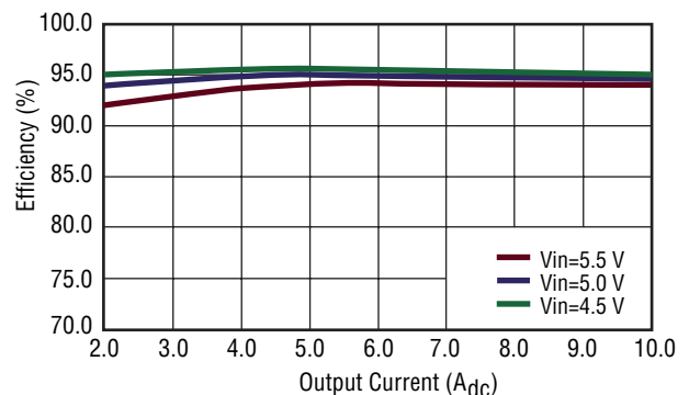
Fig. 6 Efficiency vs. Output Current ( V_{out} = 3.3 V_{dc} )
