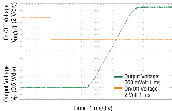
Fig. 15 Typical Start-up using Remote On/Off with Low-ESR External Capacitors (100x100 \mu F Polymer) ( V_{in} = 5.0 V_{dc} , V_o = 3.3 V_{dc} , I_o = 10.0 A , C_o = 1000 \mu F )
