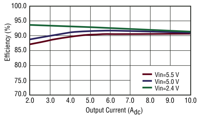
Fig. 4 Efficiency vs. Output Current ( V_{out} = 1.8 V_{dc} )
