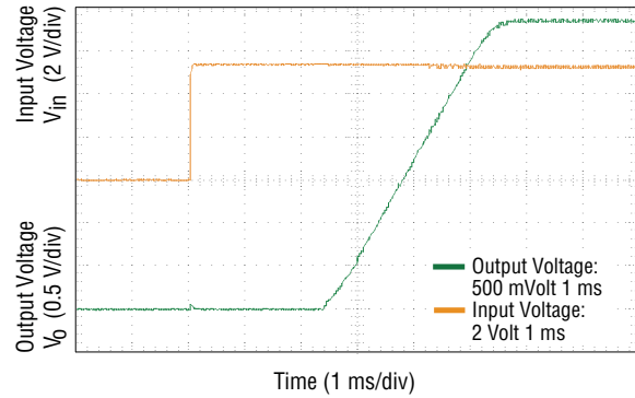
Fig. 16 Typical Start-up with Application of V_{in} ( V_{in} = 5 V_{dc} , V_o = 3.3 V_{dc} , I_o = 10 A )
