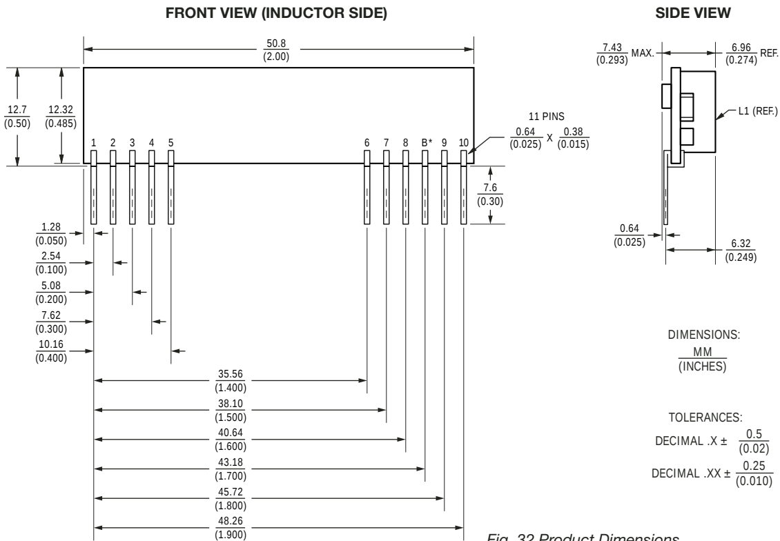
Fig. 32 Product Dimensions
