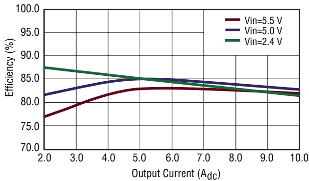
Fig. 1 Efficiency vs. Output Current ( V_{out} = 0.75 V_{dc} )
