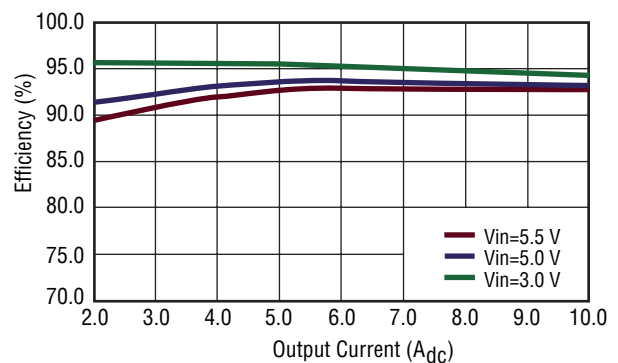
Fig. 5 Efficiency vs. Output Current ( V_{out} = 2.5 V_{dc} )
