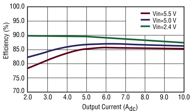
Fig. 2 Efficiency vs. Output Current ( V_{out} = 1.2 V_{dc} )
