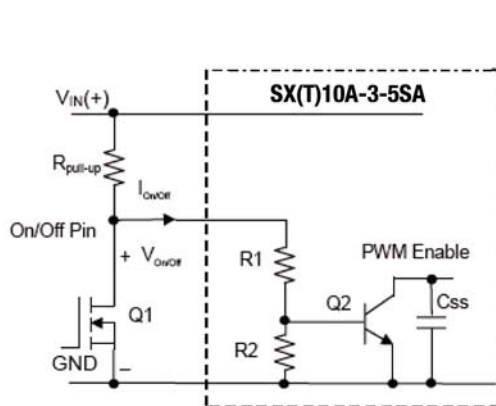
Fig. 24(a) Circuit Configuration for using Negative Logic On/Off
