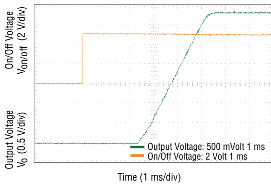
Fig. 14 Typical Start-up using Remote On/Off ( V_{in} = 5 V_{dc} , V_o = 3.3 V_{dc} , I_o = 10 A )
