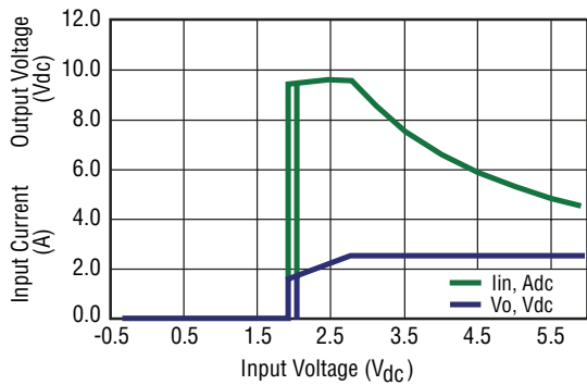
Fig. 7 Input Voltage vs. I_o and V_o ( V_o = 2.5 V_{dc} , I_o = 10.0 A )
