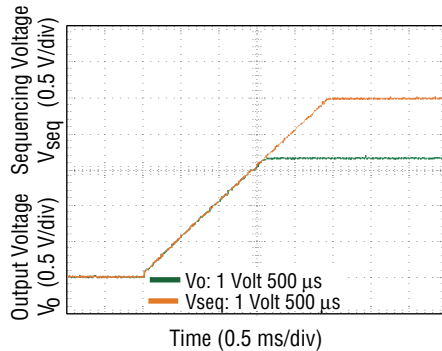
Fig. 27 Voltage Sequencing at Power Up ( V_{in} = 5.0 V_{dc} , V_O = 3.3 V_{dc} , I_O = 10.0 A )
