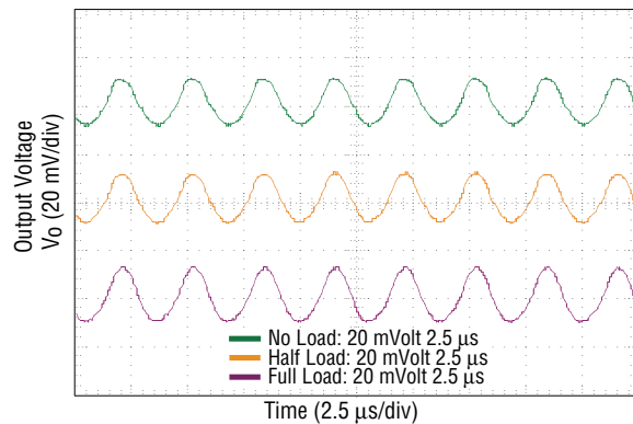
Fig. 9 Typical Output Ripple and Noise ( V_{in} = 5.0 V , V_o = 3.3 V , I_o = 10.0 A )
