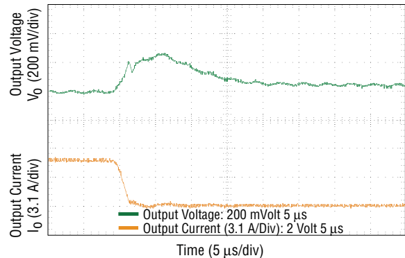
Fig. 11 Transient Response - 10 A - 5 A Step ( V_o = 3.3 V_{dc} )
