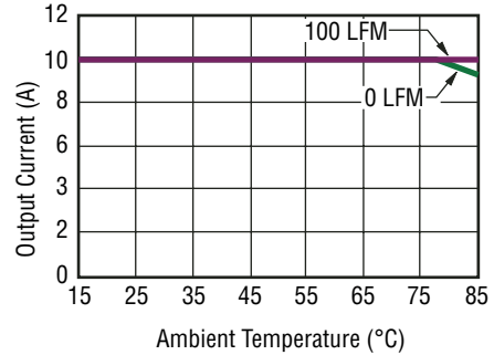
Fig. 22 Derating Output Current vs. Local Ambient Temp. and Airflow (V_{in} = 5.0 V_{dc}, V_o = 3.3 V_{dc})
