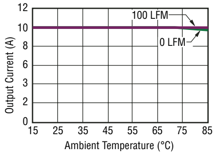
Fig. 19 Derating Output Current vs. Local Ambient Temp. and Airflow (V_{in} = 5.0 V_{dc}, V_o = 0.75 V_{dc})
