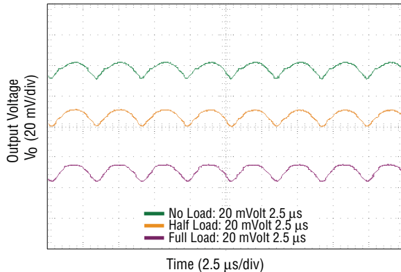
Fig. 8 Typical Output Ripple and Noise ( V_{in} = 5.0 V , V_o = 0.75 V , I_o = 10.0 A )
