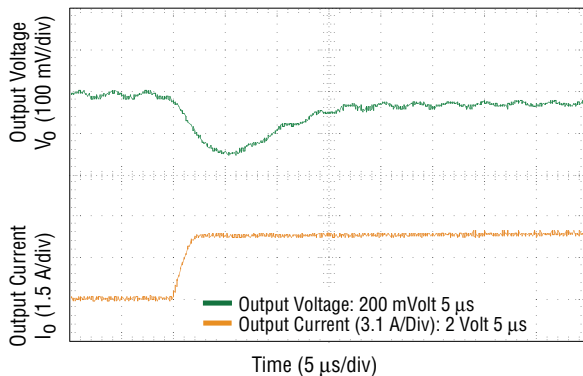
Fig. 12 Transient Response - 5 A - 10 A Step ( V_o = 3.3 V_{dc} , C_{ext} = 3 \times 100 \mu F Polymer Capacitors)
