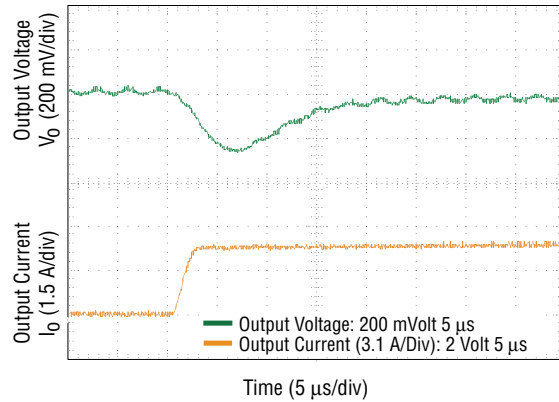
Fig. 10 Transient Response - 5 A - 10 A Step ( V_o = 3.3 V_{dc} )
