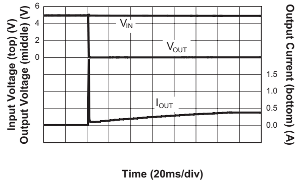
Hard Short Circuit ( V_{IN} = 5V )
