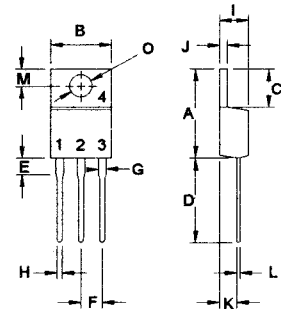
TO-220
