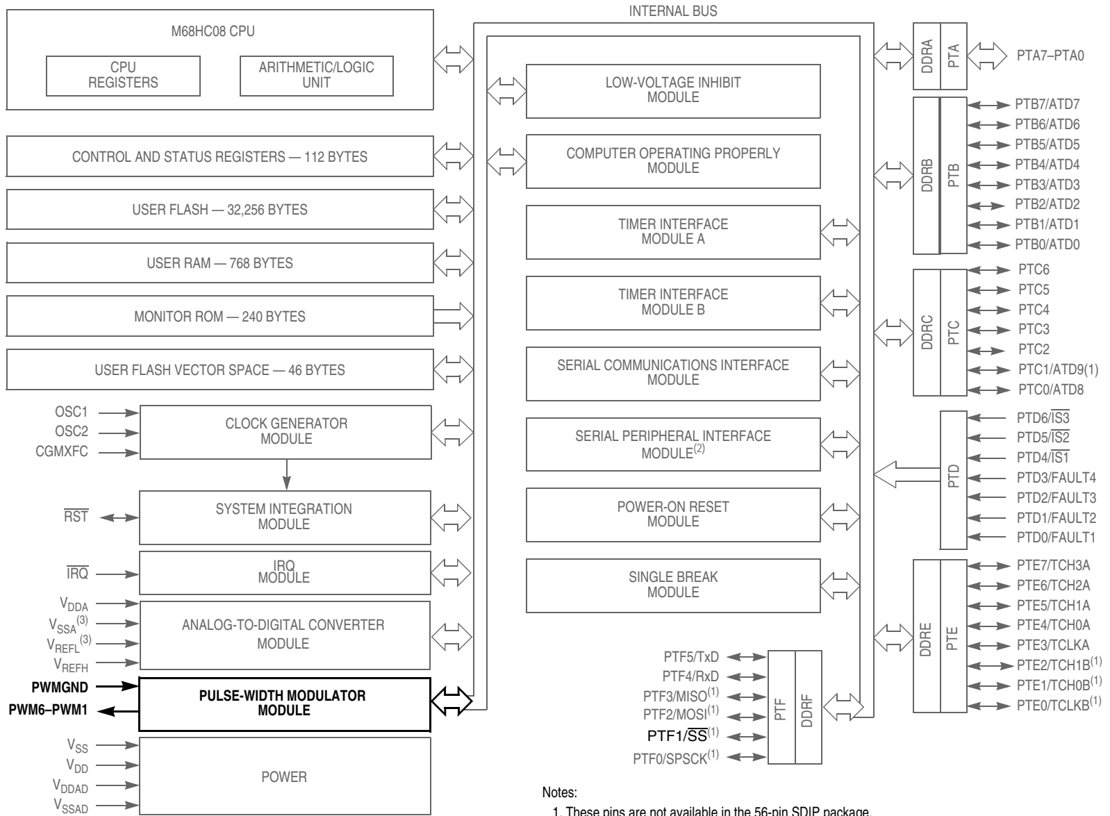
Figure 12-1. Block Diagram Highlighting PWM6 Block and Pins
