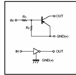
●Equivalent circuit
