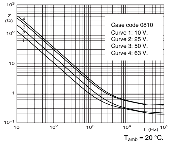
Fig.8 Typical impedance as a function of frequency.
