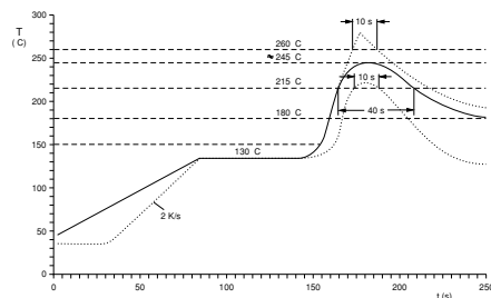
Reflow soldering.
