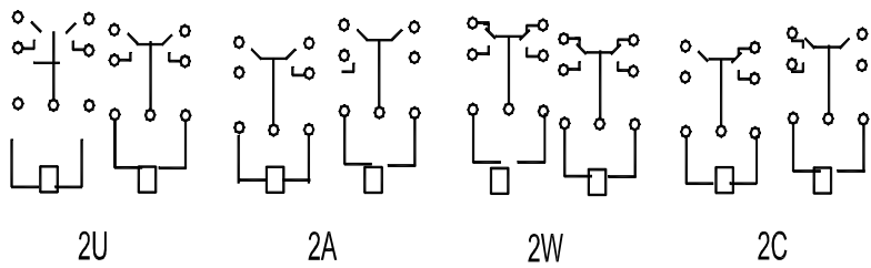
Wiring diagram(Bottom views)
