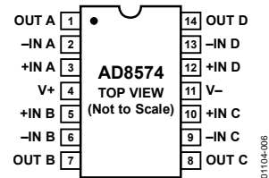
Figure 6. 14-Lead SOIC (R Suffix)
