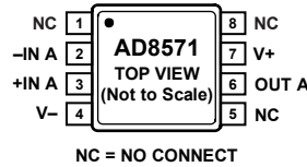
Figure 1. 8-Lead MSOP (RM Suffix)
