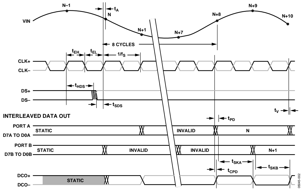
Figure 2. Timing Diagram
