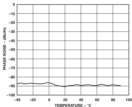
TPC 16. IF Phase Noise vs. Temperature (540 MHz, 200 kHz, 20 kHz)
