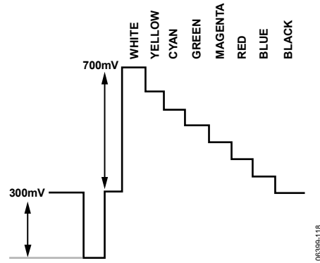
Figure 117. Y Levels—PAL
