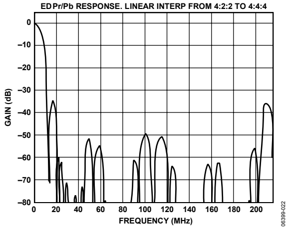
Figure 22. ED 8x Oversampling, PrPb Filter (Linear) Response
