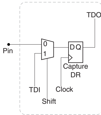
Pin BSC
