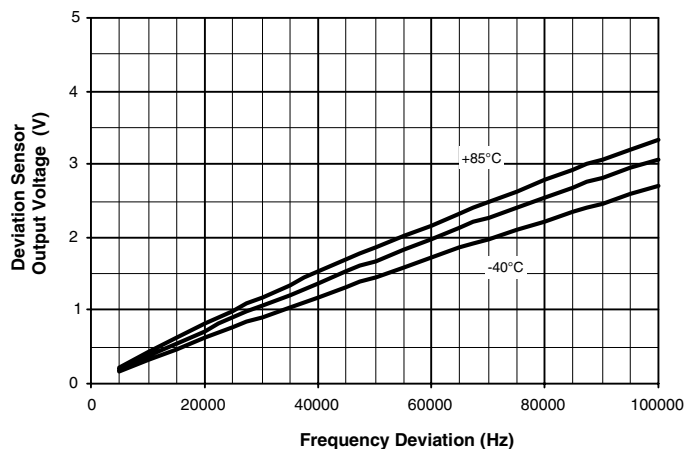
Figure 15. Deviation Sensor
