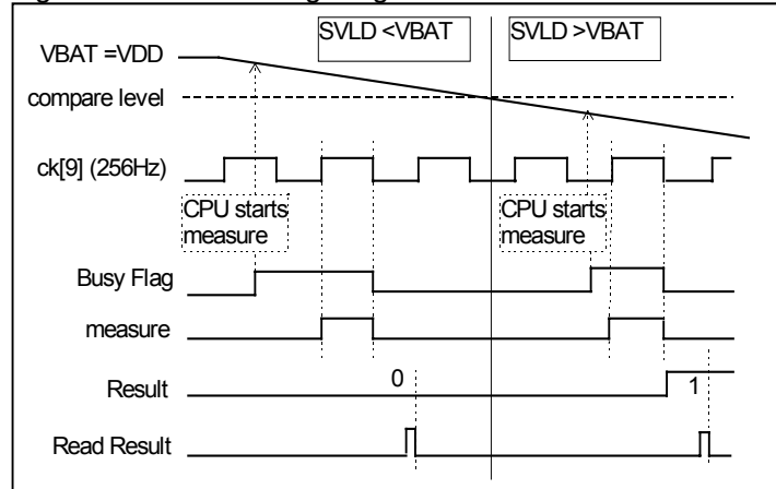
Figure 23. SVLD Timing Diagram
