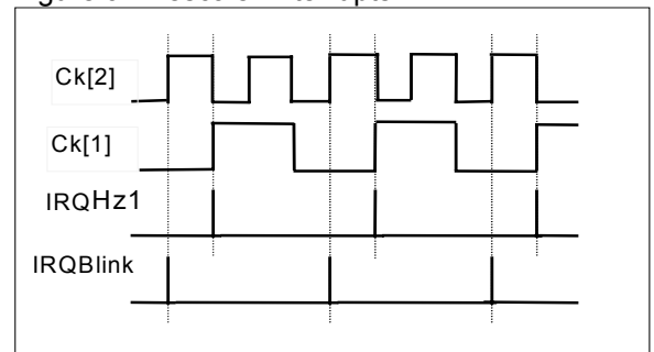
Figure 9. Prescaler Interrupts
