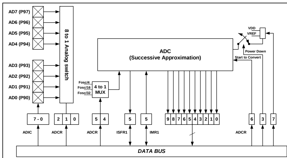
Fig. 5-5 AD Converter
