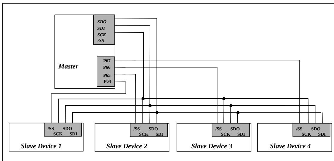
Fig. 5-17 The SPI Configuration Example of Single-Master and Multi-Slaves
