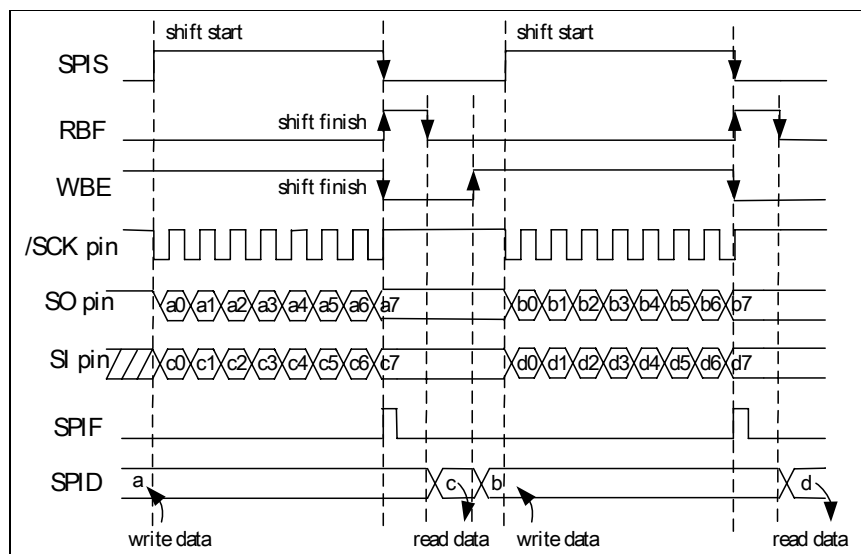
Fig. 5-16 Transmit/Receive Mode (8-bit, 1 word)
