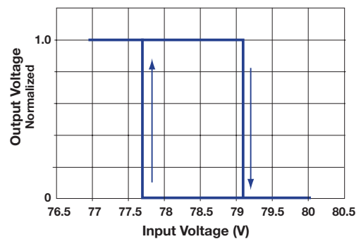
Overvoltage Hysteresis
