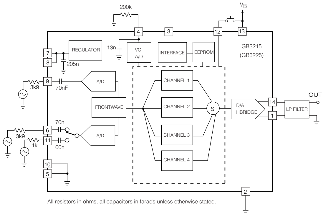
Figure 1: Test Circuit
