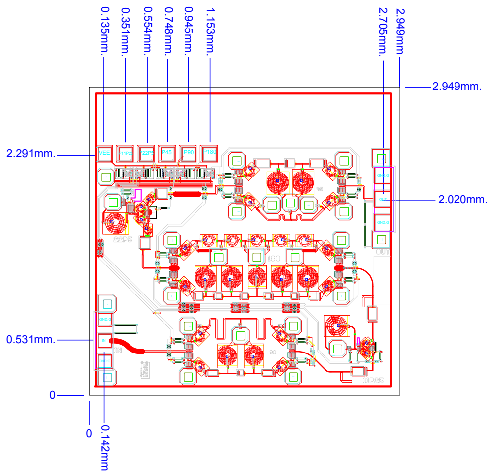
Figure 7. Die Layout
