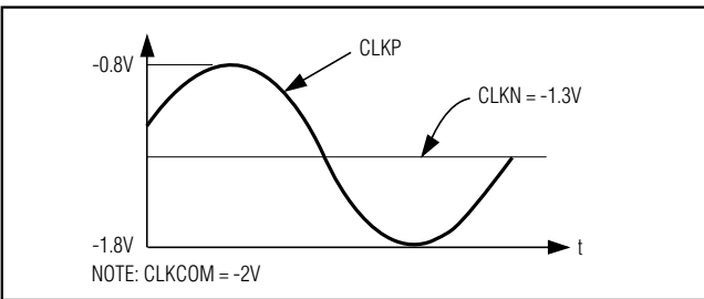
Figure 13c. Single-Ended Clock Input—ECL Drive
