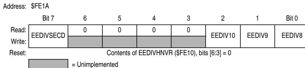
Figure 2-6. EEDIV Divider High Register (EEDIVH)
