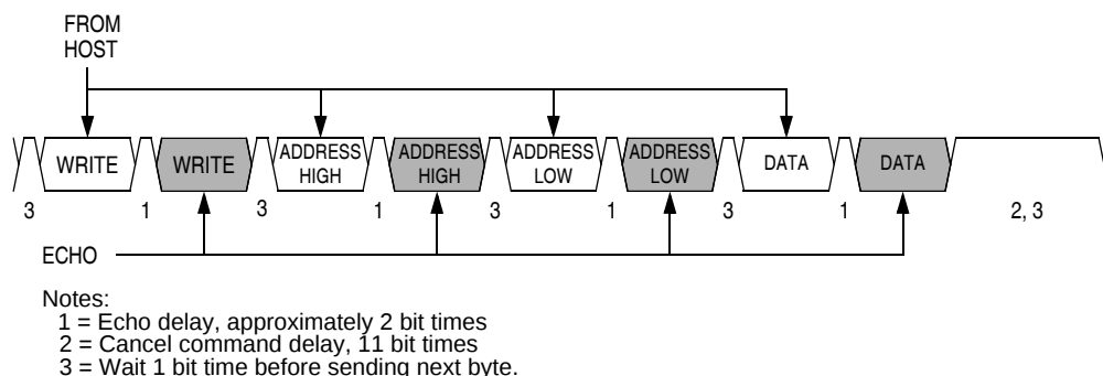
Figure 17-11. Write Transaction
