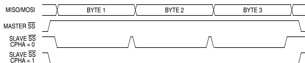
Figure 15-13. CPHA/SS Timing
