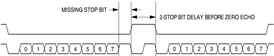
Figure 17-9. Break Transaction
