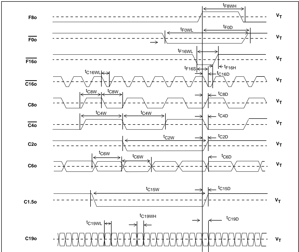
Figure 12 - Output Timing 1
