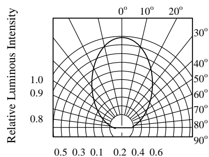
FIG.6 RADIATION DIAGRAM
