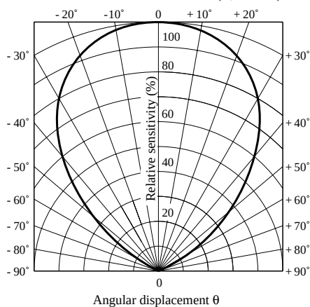
Fig. 8 Radiation Diagram ( T_a = 25^\circ C )
