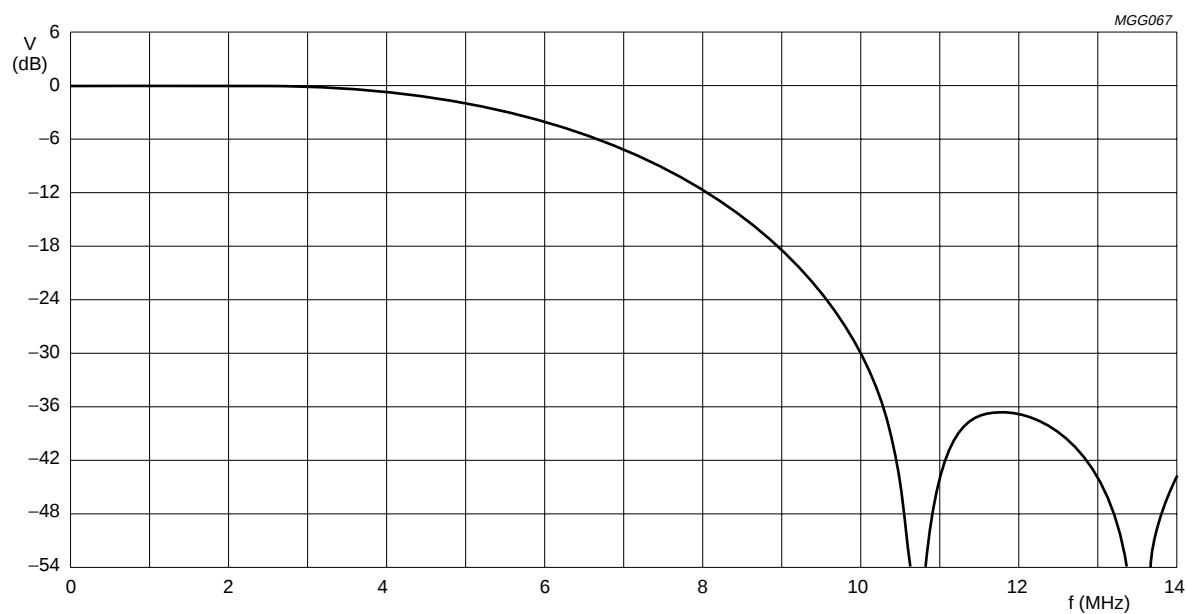
Fig.22 Interpolation filter for the upsampled CVBS signal.
