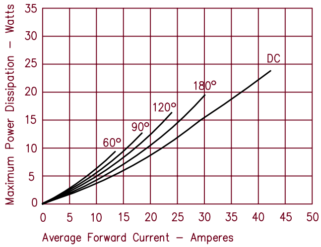
Figure 6 Maximum Forward Power Dissipation – Standard Polarity
