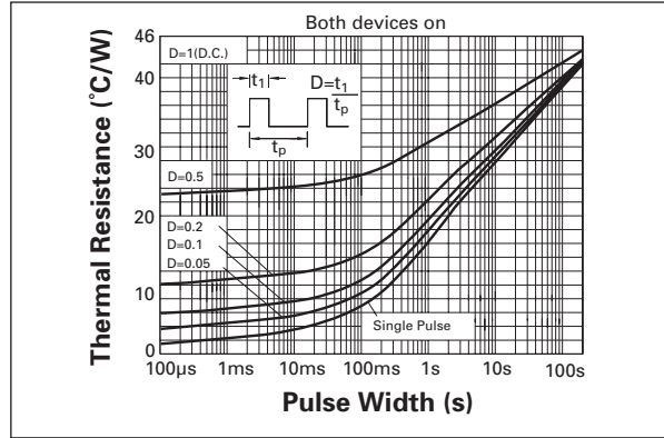
Both die on 2.75W Devices
