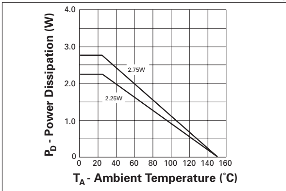
2.25W and 2.75W Derating
