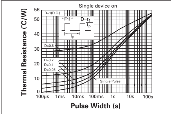
Single die on 2.25W Devices
